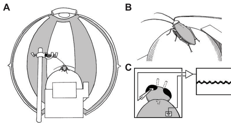
Fig. 1. The virtual reality setup. (A) A fisheye lens on top projects the images of black and white bars from the projector above it (not shown) onto the inner surface of the spherical screen. The trackball system is placed inside the sphere so that the cockroach is at the equator of the sphere. (B) The placement of the animal on the trackball. (C) Electrode placement in the preparation during intracellular recordings. Dashed line shows where the antennae of an intact cockroach would be. For more detailed information, see Takalo et al. (Takalo et al., 2012).
